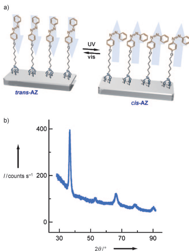
Figure 1. a) Representation of the hybrid films and their preparation procedures. The AZ monolayer was formed on the surface of the Nb film by immersing the bare Nb film into AZ solution for 48 h. The arrows show the direction of the surface dipole layer, which arises from cooperative effects of the intrinsic molecular dipole moment. b) GIXD patterns of a bare Nb film on a glass substrate. The five peaks that are observed for (110), (200), (211), (220), (310) are consistent with a face-centered cubic crystal structure of Nb with lattice constant a = 3.29 \text{ \AA} , which is ca. 5 % smaller than the corresponding value for bulk Nb ( 3.45 \text{ \AA} ).
