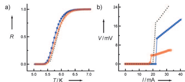
Figure 3. a) Temperature dependence of the resistance of the hybrid film for the initial state (dashed line), the UV photostationary state (filled blue circles) and the visible photostationary state (open red circles). Resistance values are normalized. b) V – I measurements of the hybrid film for the initial state (dashed line), the UV photostationary state (filled blue circles), and the visible photostationary state (open red circles) at 2 K.
