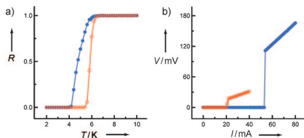
Figure 2. a) Temperature dependence of the Nb film resistance before (filled blue circles) and after (open red circles) the surface passivation of the AZ monolayer. Resistance values are normalized. b) V – I measurements of the Nb film before and after the surface passivation of the AZ monolayer at 2 K. The I_c value of 53 mA for the bare Nb film (filled circles) decreased to 20 mA after surface passivation (open circles).
