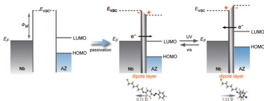
Figure 4. Changes in the work function arising from the photoisomerization of AZ. Schematic energy level diagrams for an untreated interface (without surface passivation; left); passivation of trans -AZ imposes an interface dipole that decreases the local vacuum energy level ( E_{vac} ; center); photoisomerization to cis -AZ imposes an interface dipole that increases the local vacuum energy level ( E_{vac} ; right).
